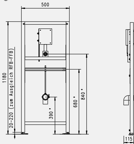
Urinal-Element
