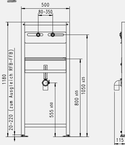
Urinal-Element
