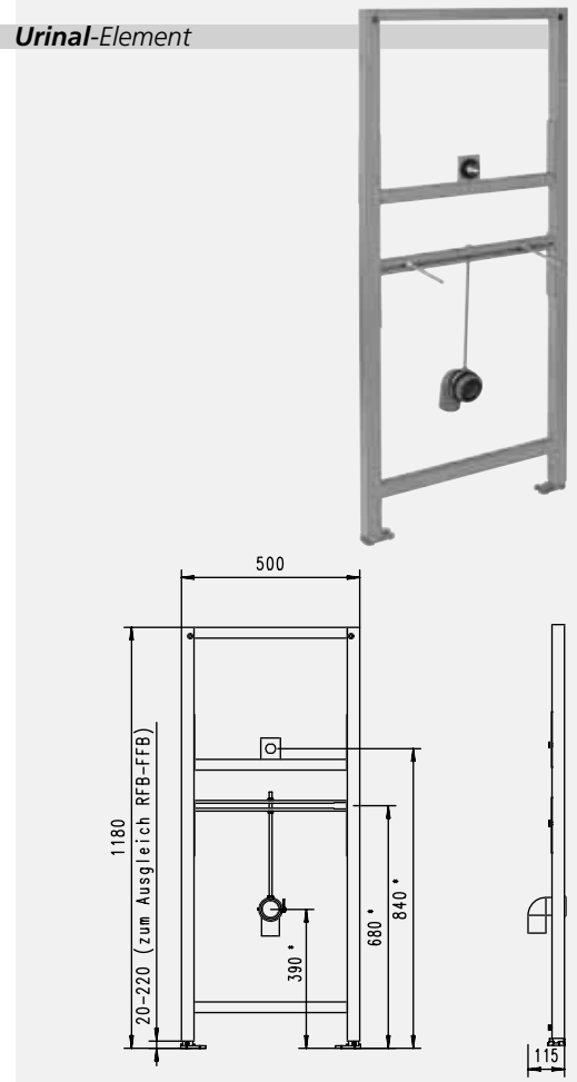
Urinal-Element
