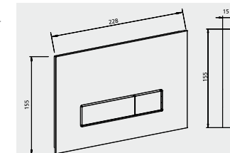
AMBIENTE Schiefer, grau / glanz verchromt Art.-Nr. 167-3300SCSW-00
